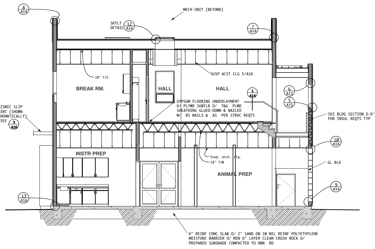
SECTION B - B 1/4" = 1'-0"
