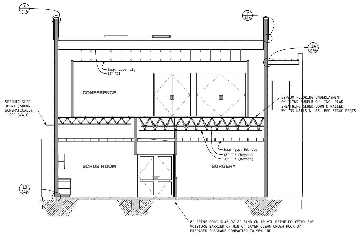
SECTION A - A 1/4" = 1'-0"
