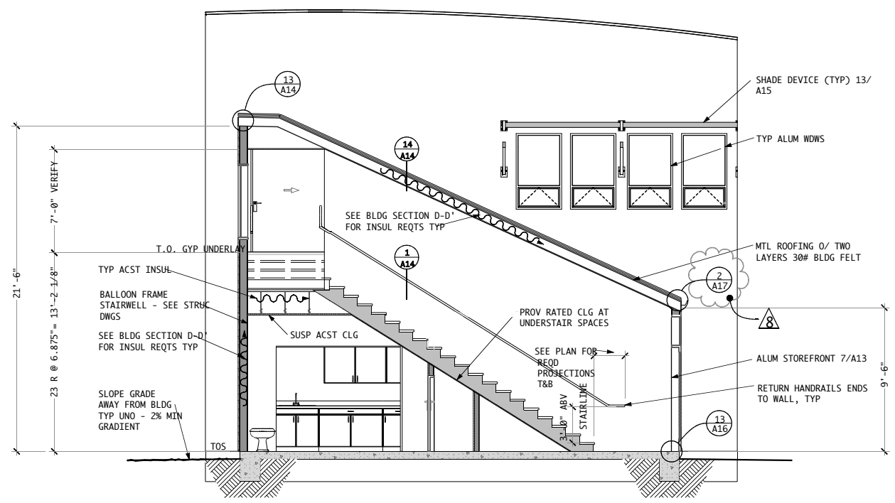
SECTION A - A 1/4" = 1'-0"
